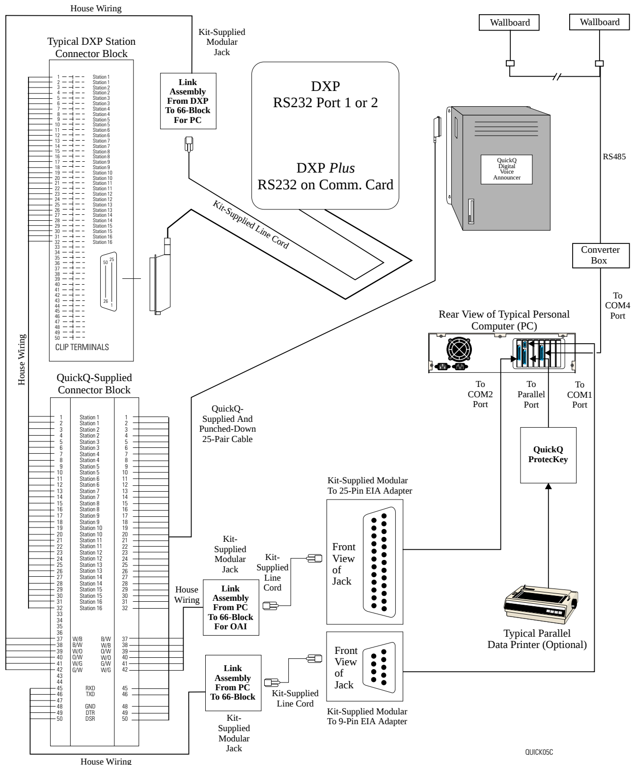
Figure 3-8. Reviewing The System Interconnection
