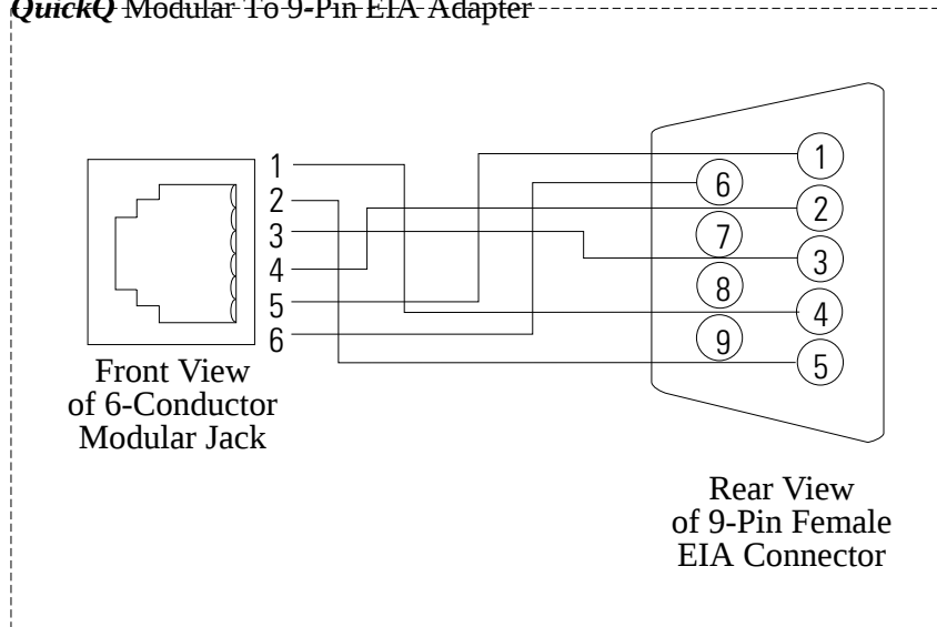
QuickQ Modular To 9-Pin EIA Adapter
