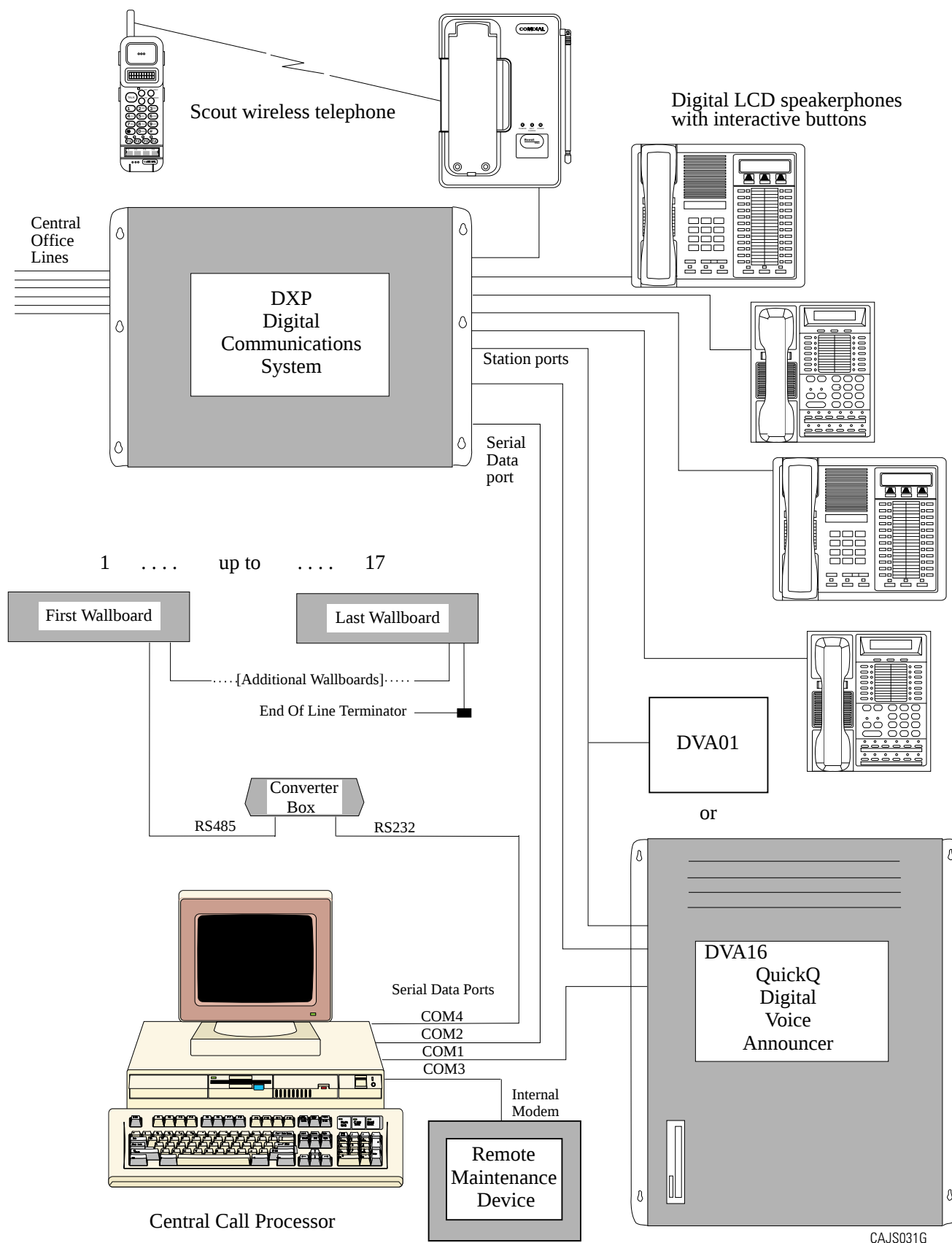
Figure 1-1. Overviewing The QuickQ System
