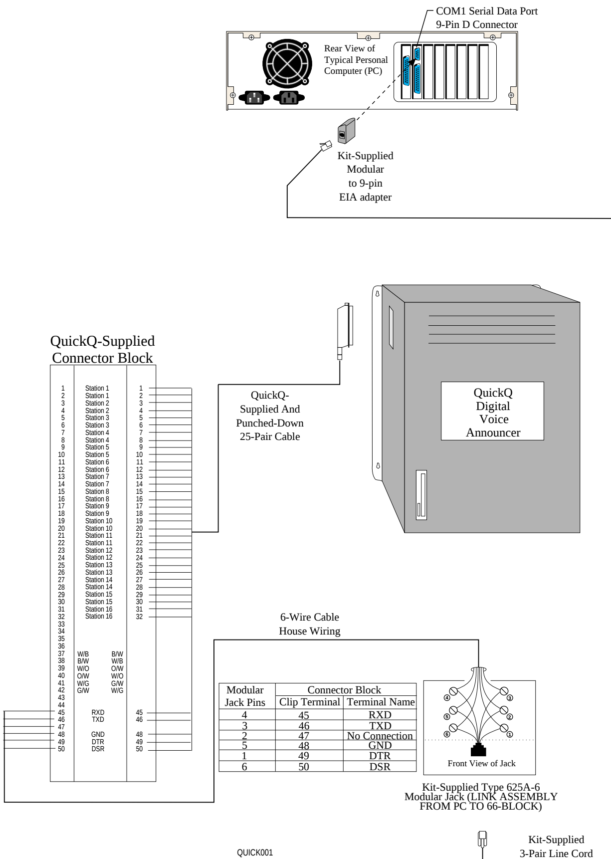
Figure 3-2. Connecting The Personal Computer To The DVA
